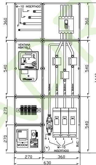
TMF-10 80...160 A
