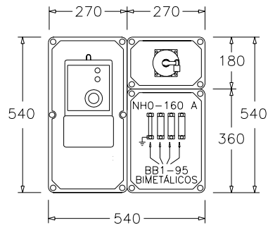
TMF1-ST
